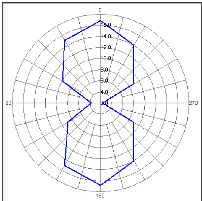
Read range (in meter) at various angle
